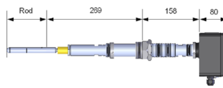
Passive/Active Sensor 0-250°C
