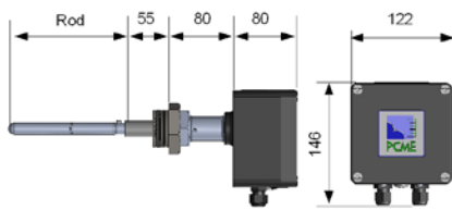
Standard Sensor 0-250°C
